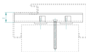
Universalanker Staffa universale Universal bracket
